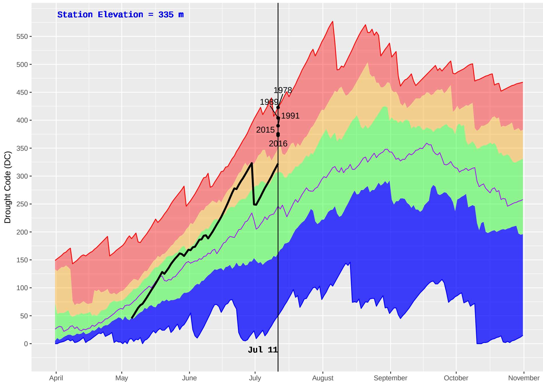
KISPIOX HUB (428) : Historical (1970–2016) and Current (2018) Noon Drought Code (DC)
