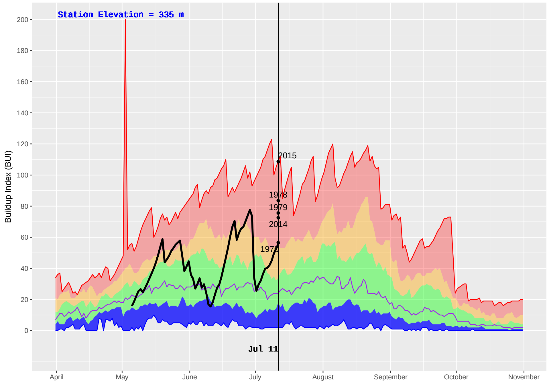
KISPIOX HUB (428) : Historical (1970–2016) and Current (2018) Noon Buildup Index (BUI)
